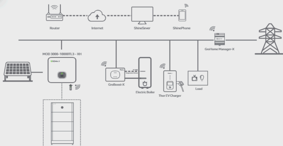
GroHome System Diagram
