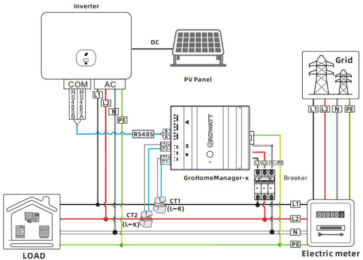
Figure 22 Splitting system
