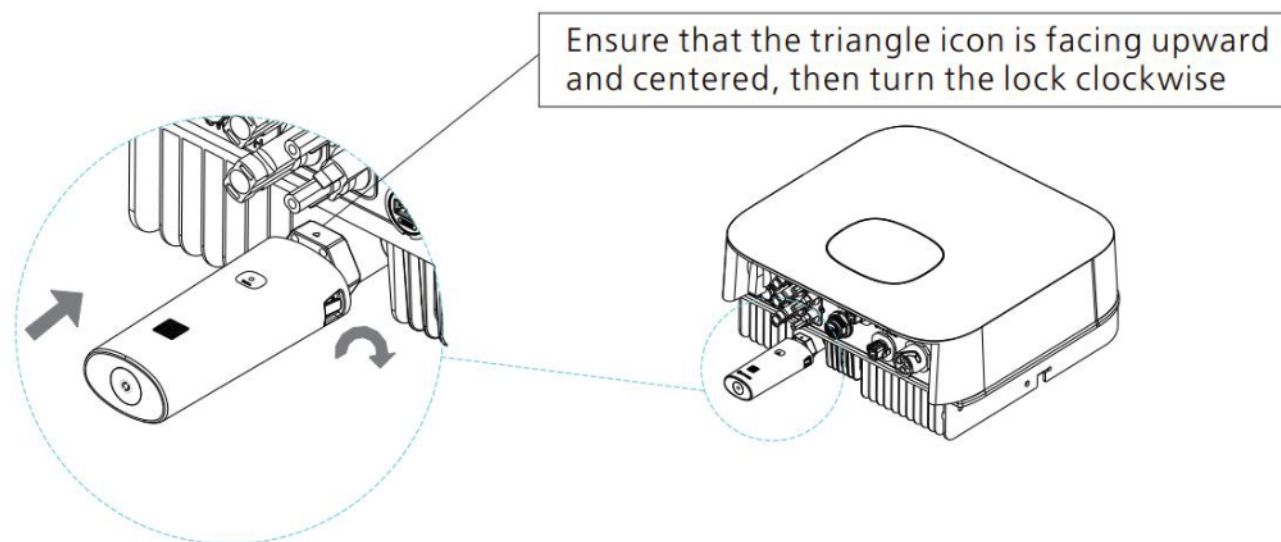
Figure 17 ShineRFStick-X2 slave mounting
