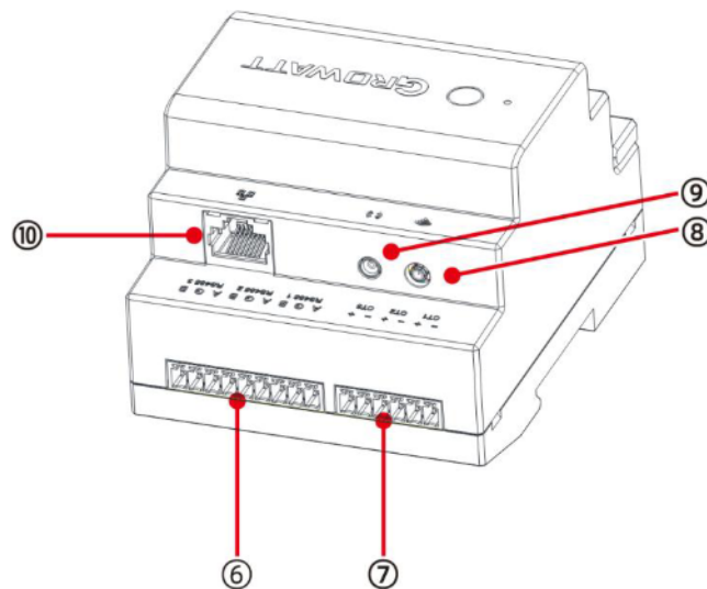
Figure 4 GroHomeManager-X Communication Module
