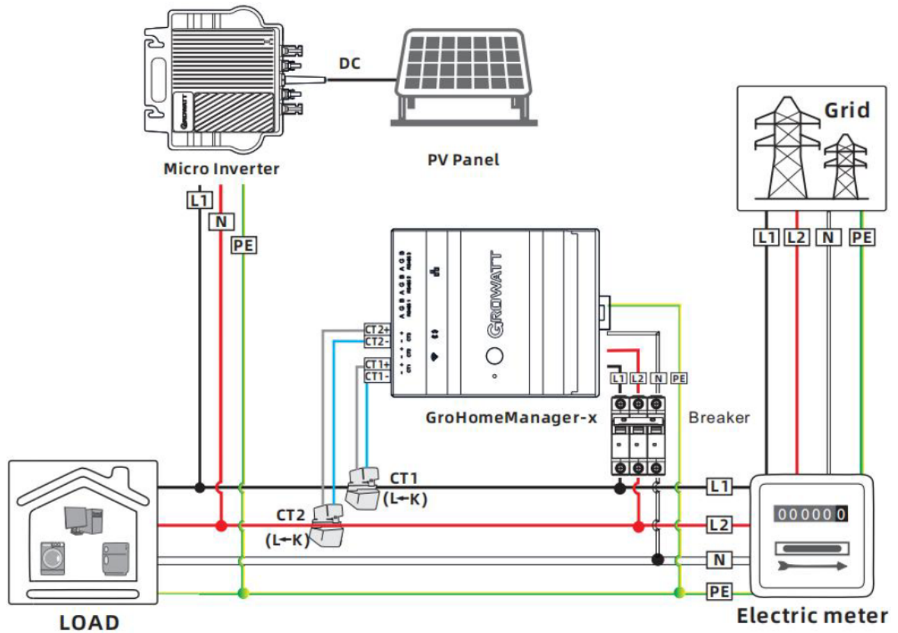
Figure 21 Split phase inverse system
