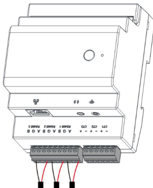
Figure 12 GroHomeManager-X Install the RS485 port
