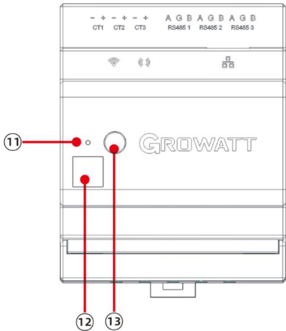
Figure 5 GroHomeManager-X User interaction module
