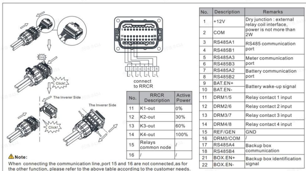
Figure 13 MID/MOD-XH RS485 wiring diagram
