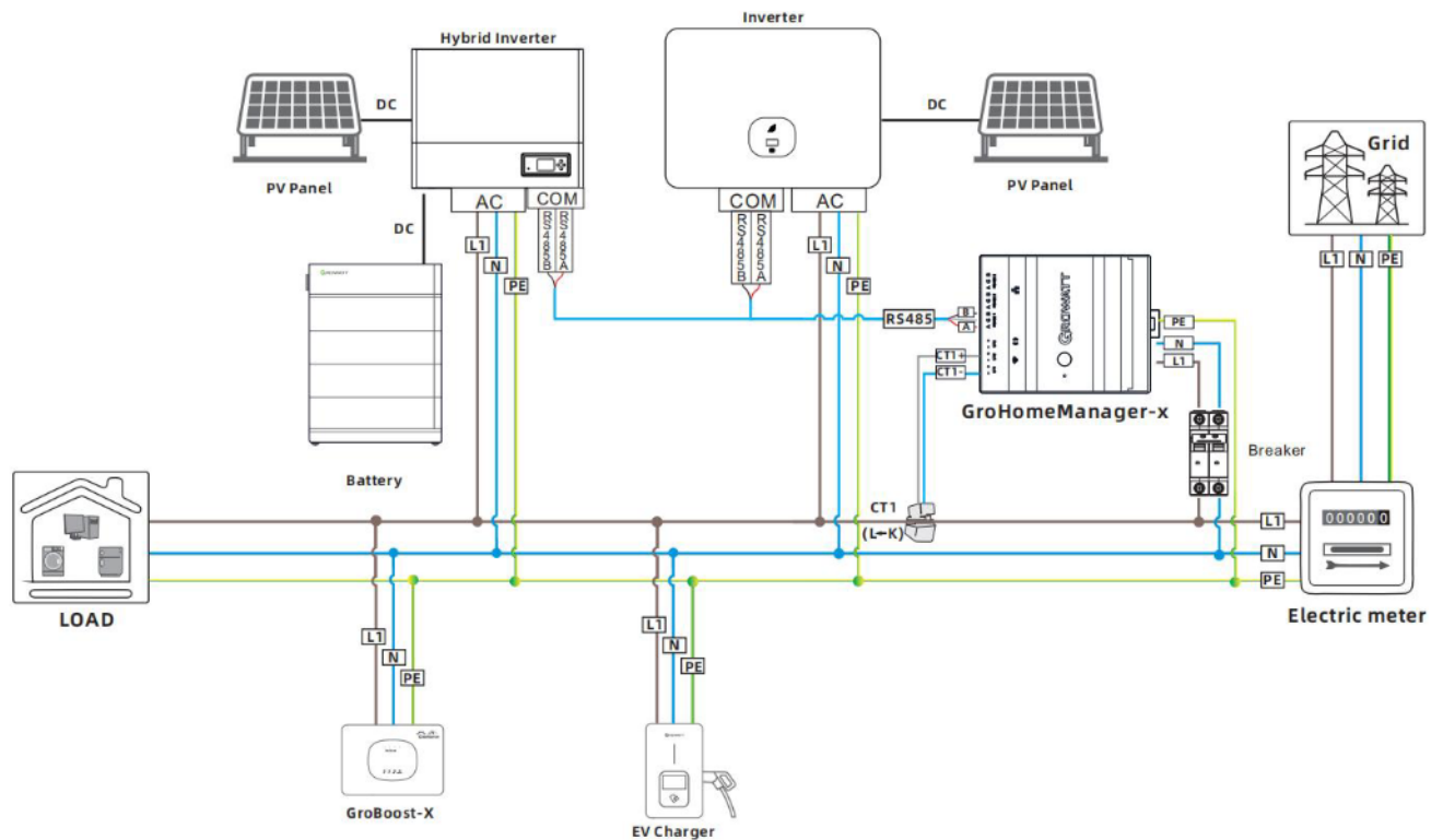
Figure 20 Single-phase HEMS system
