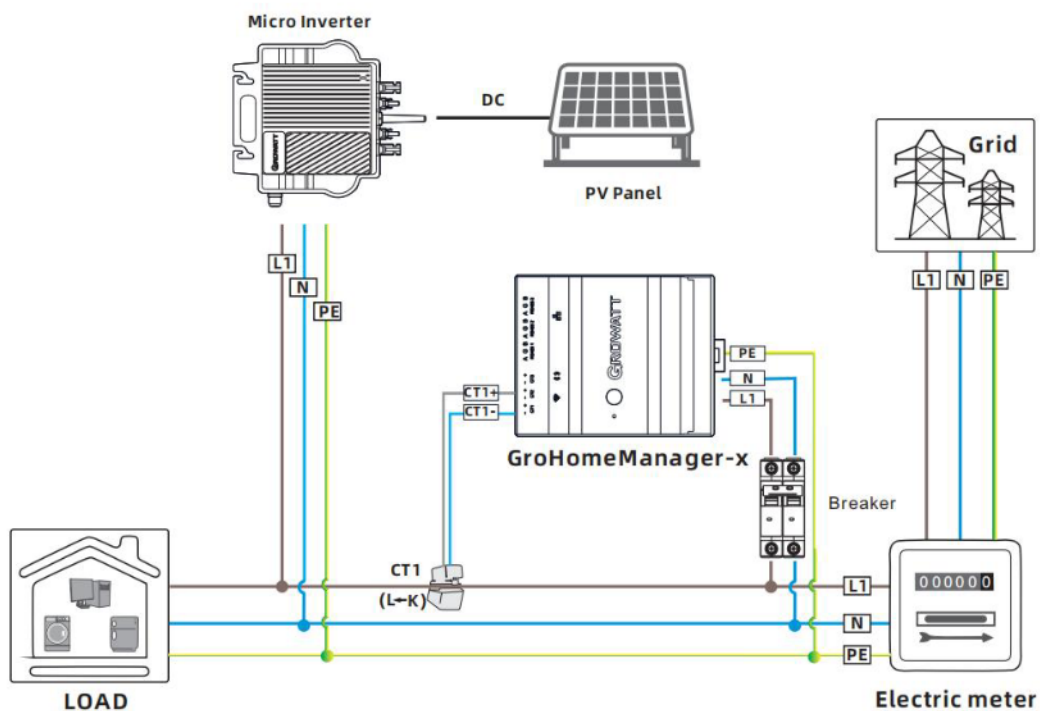
Figure 19 Single-phase micro-inverse grid-connected anti-backflow system
