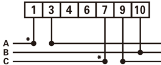
Figure13 Three phase three wire: direct connect
