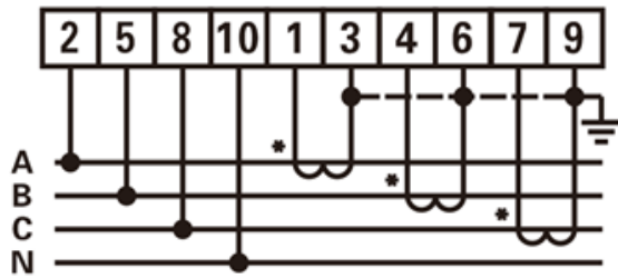
Figure14 Three phase four wire: via current transformer
