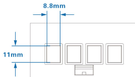
Figure9 current cable terminal (Conductor Cross-sectional Area Range \leq 16 \text{ mm}^2 )
