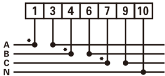
Figure12 Three phase four wire: direct connect
