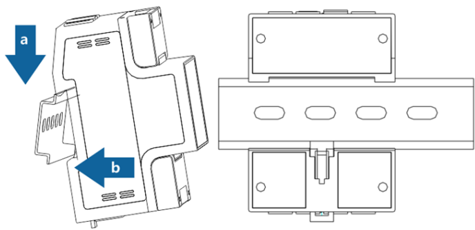
Figure11 Installation Diagram
