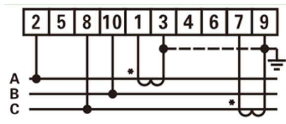
Figure15 Three phase three wire: via current transformer
