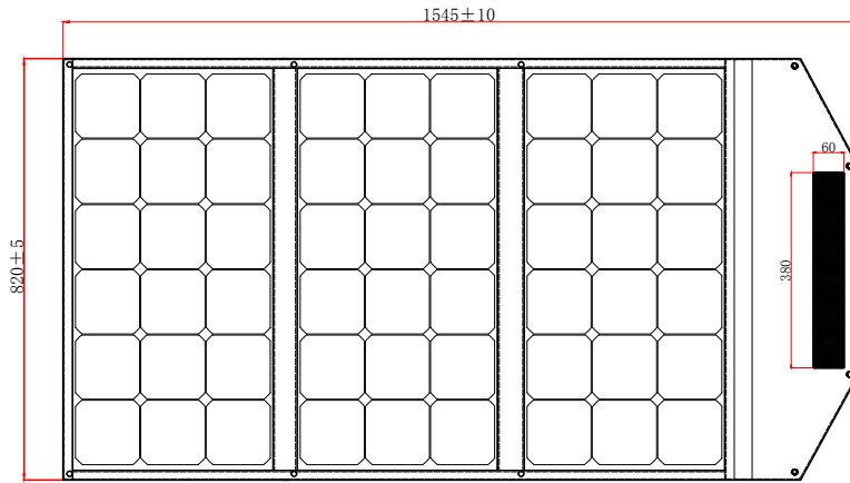
3*65W33.5v charging pack front view
