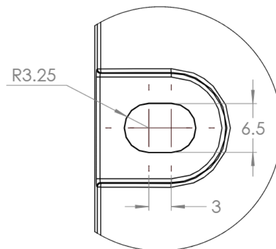
DETAIL A (4x) SCALE 2 : 1
